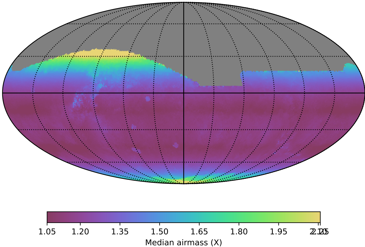
too_combined_s0.5_v3.4_10yrs All sky r band: Median airmass
