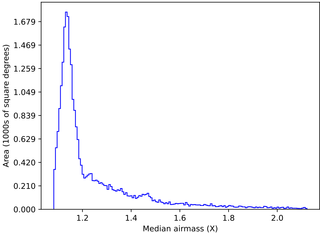
too_combined_s0.5_v3.4_10yrs All sky r band: Median airmass
