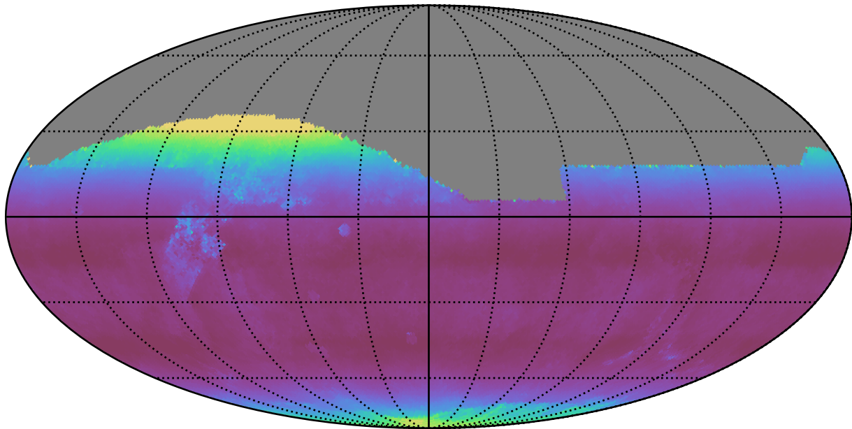
too_combined_s0.5_v3.4_10yrs All sky i band: Median airmass
