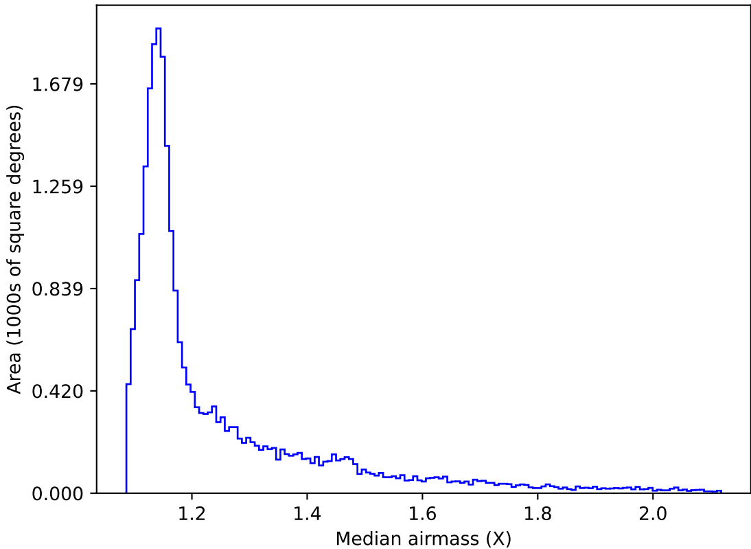
too_combined_s0.5_v3.4_10yrs All sky i band: Median airmass
