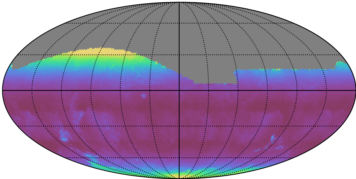
too_combined_s0.5_v3.4_10yrs All sky g band: Median airmass
