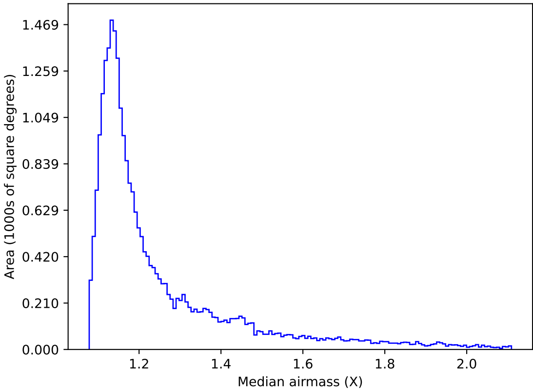
too_combined_s0.5_v3.4_10yrs All sky g band: Median airmass
