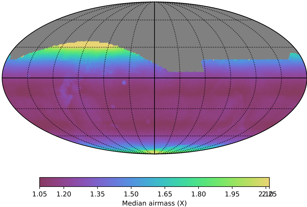
too_combined_s0.5_v3.4_10yrs All sky all bands: Median airmass
