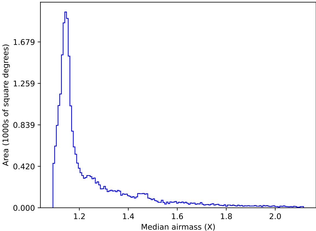
too_combined_s0.5_v3.4_10yrs All sky all bands: Median airmass
