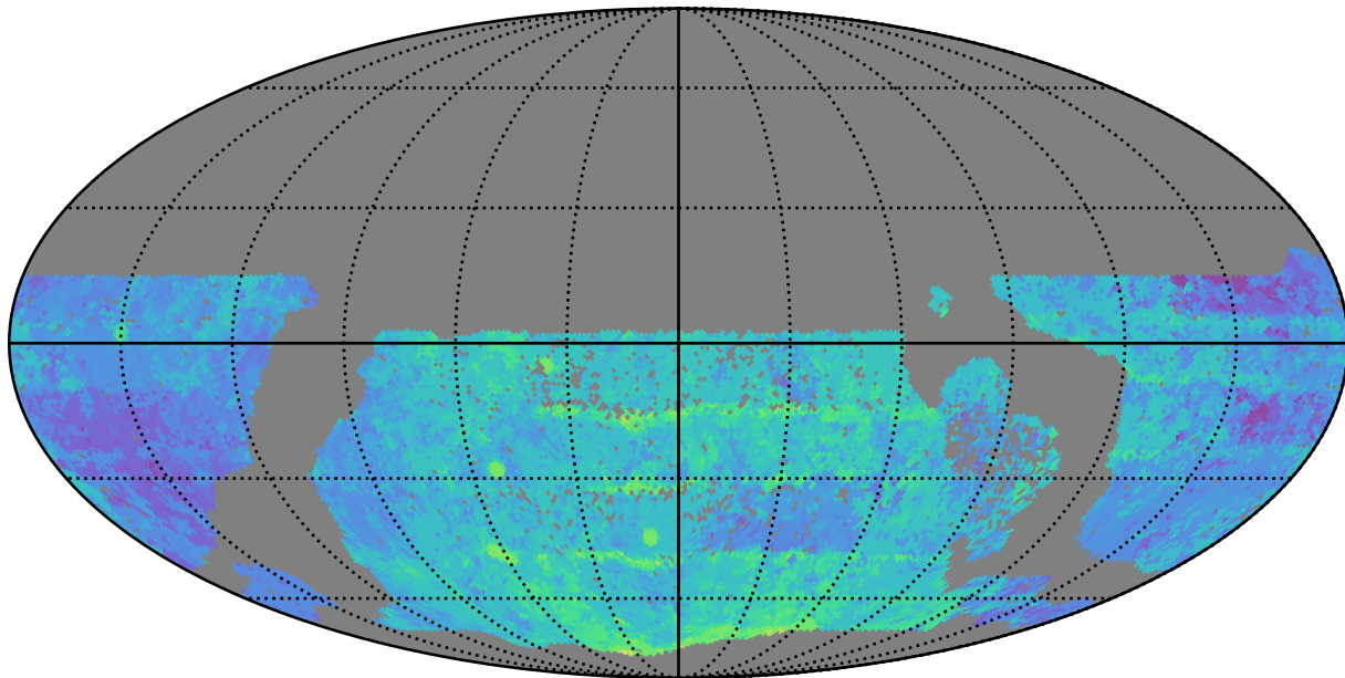
too_combined_s0.5_v3.4_10yrs WFD y band: Median Season Length
