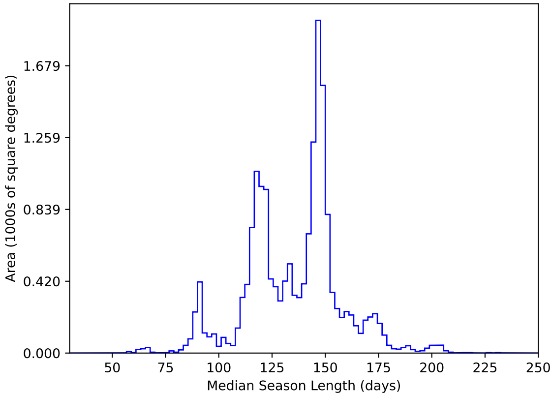
too_combined_s0.5_v3.4_10yrs WFD y band: Median Season Length
