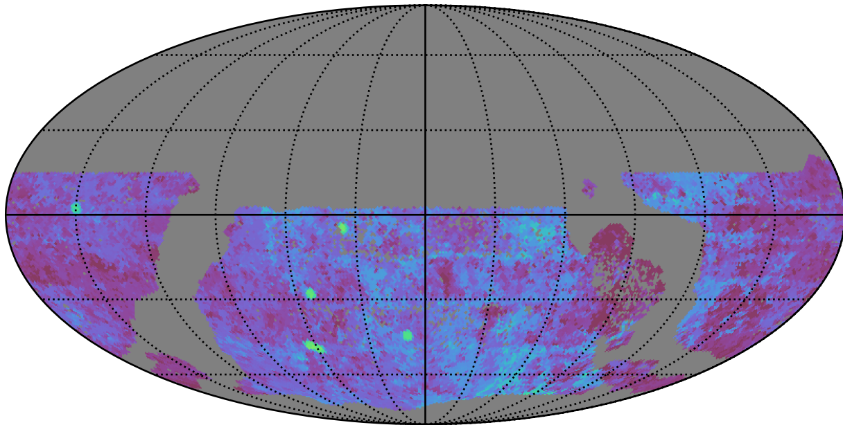
too_combined_s0.5_v3.4_10yrs WFD u band: Median Season Length
