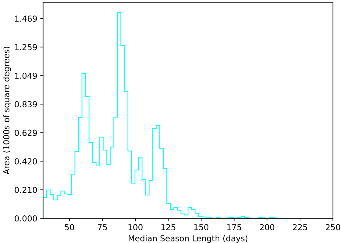
too_combined_s0.5_v3.4_10yrs WFD u band: Median Season Length
