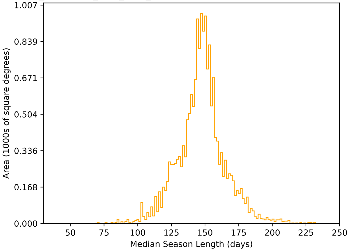
too_combined_s0.5_v3.4_10yrs WFD r band: Median Season Length
