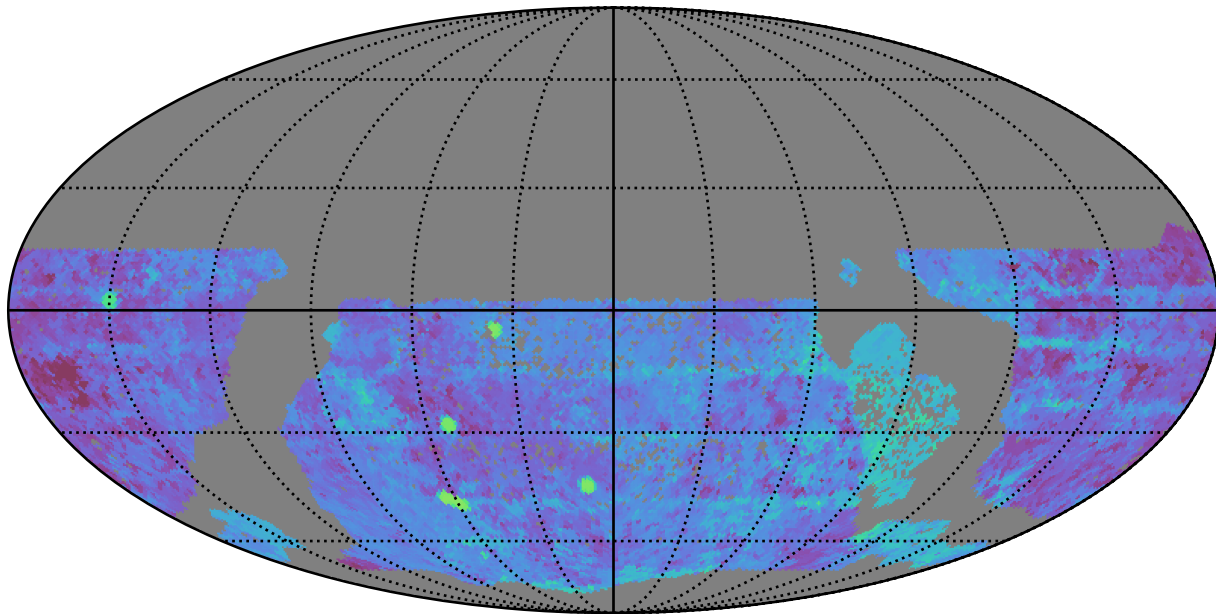
too_combined_s0.5_v3.4_10yrs WFD g band: Median Season Length
