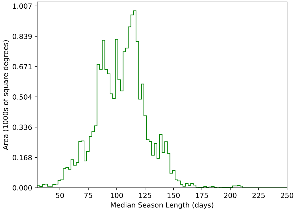
too_combined_s0.5_v3.4_10yrs WFD g band: Median Season Length
