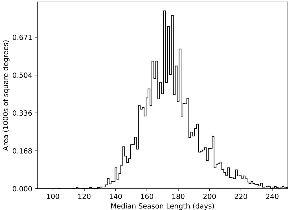
too_combined_s0.5_v3.4_10yrs WFD all bands: Median Season Length
