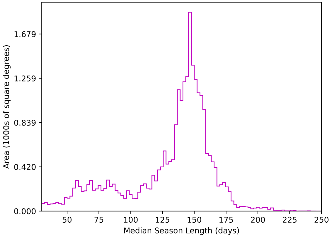
too_combined_s0.5_v3.4_10yrs All sky z band: Median Season Length
