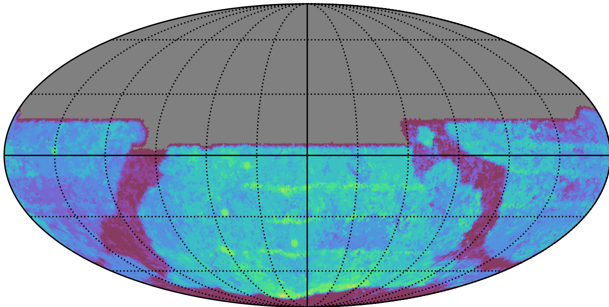
too_combined_s0.5_v3.4_10yrs All sky y band: Median Season Length
