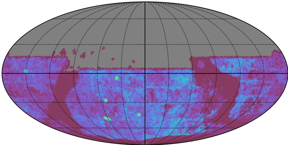
too_combined_s0.5_v3.4_10yrs All sky u band: Median Season Length
