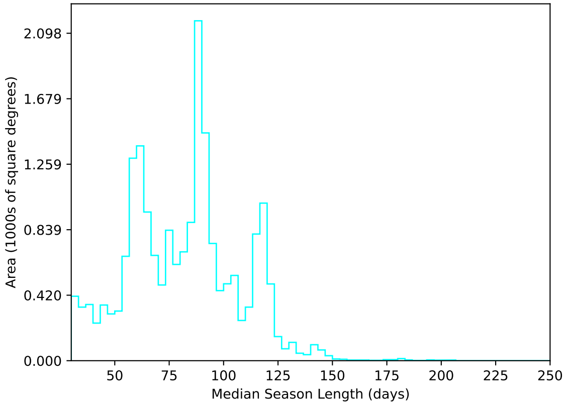
too_combined_s0.5_v3.4_10yrs All sky u band: Median Season Length
