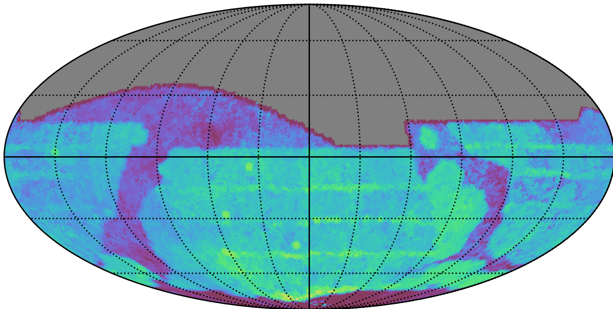
too_combined_s0.5_v3.4_10yrs All sky r band: Median Season Length
