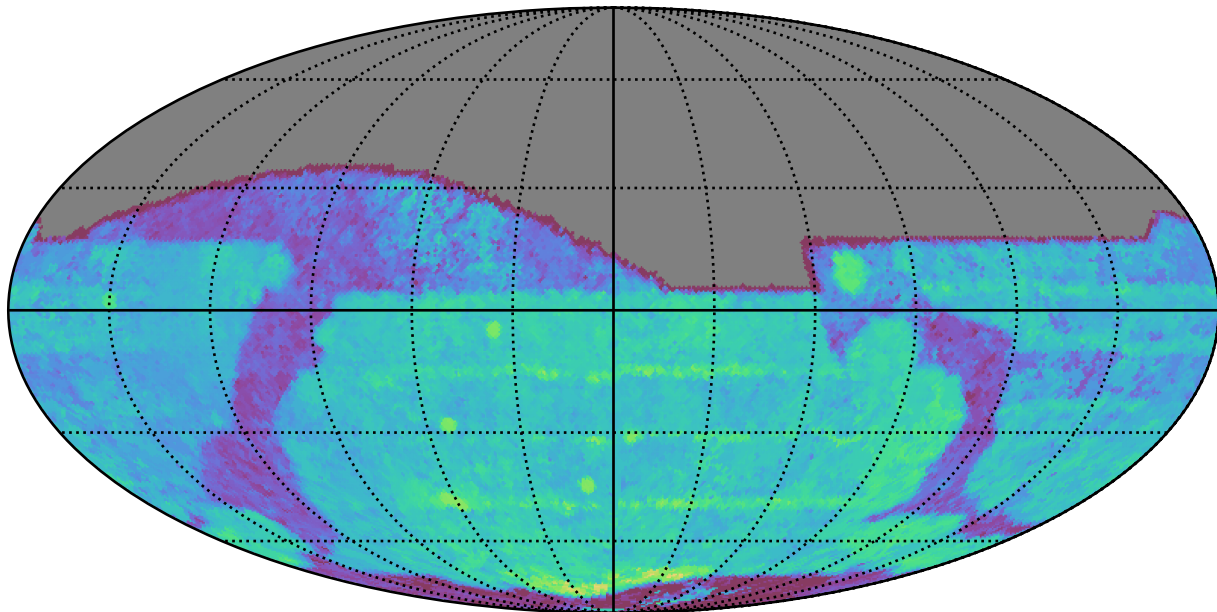
too_combined_s0.5_v3.4_10yrs All sky i band: Median Season Length
