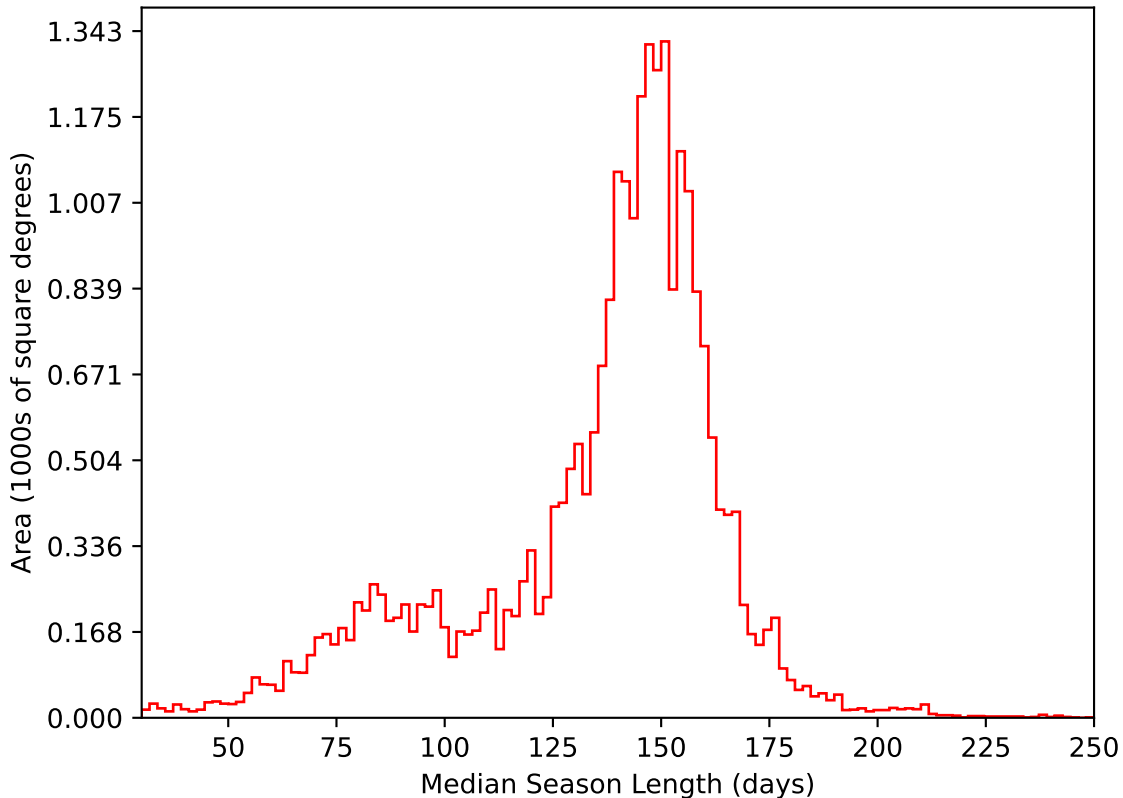
too_combined_s0.5_v3.4_10yrs All sky i band: Median Season Length
