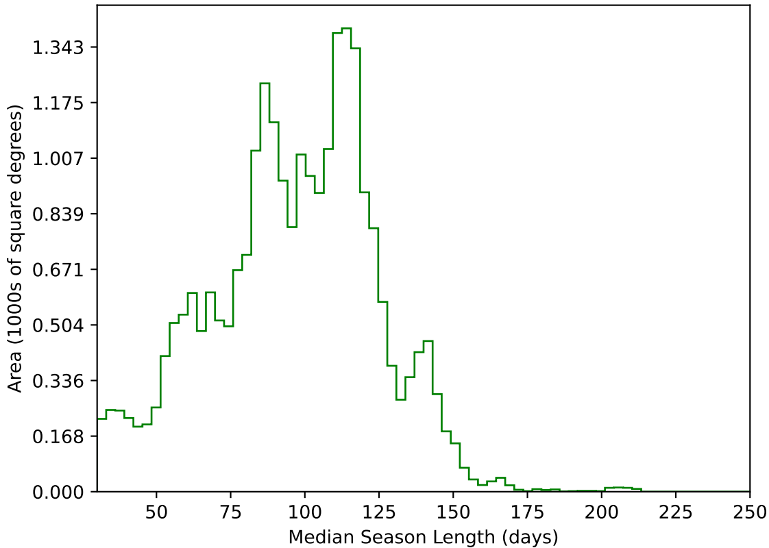
too_combined_s0.5_v3.4_10yrs All sky g band: Median Season Length
