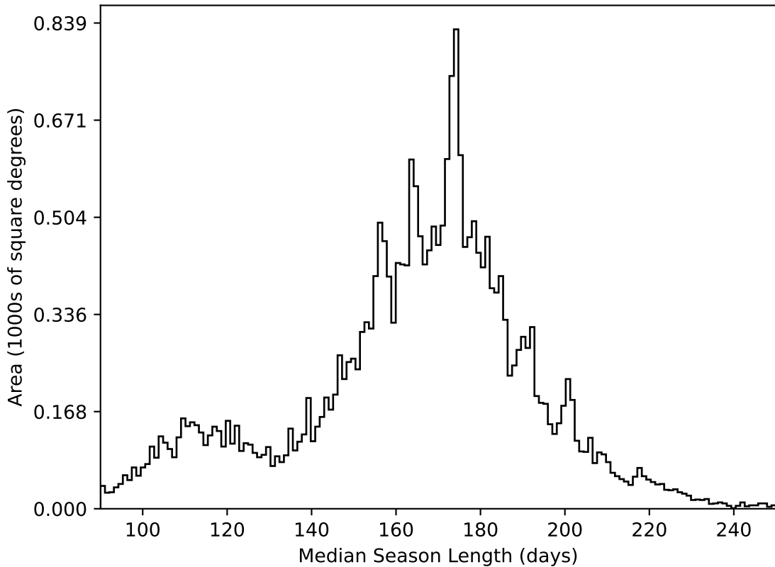
too_combined_s0.5_v3.4_10yrs All sky all bands: Median Season Length
