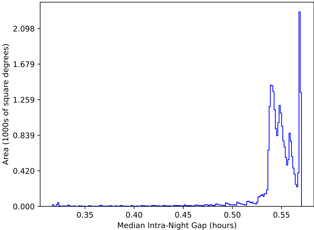
too_combined_s0.5_v3.4_10yrs All sky: Median Intra-Night Gap
