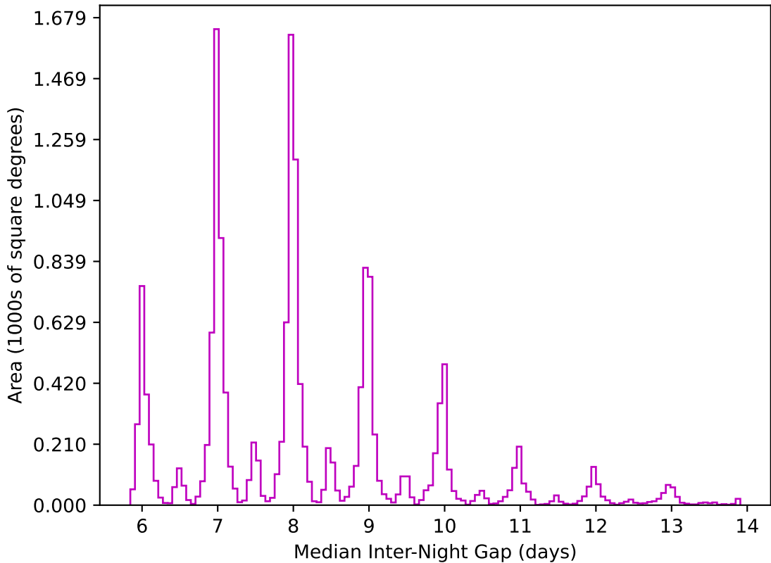
too_combined_s0.5_v3.4_10yrs WFD z band: Median Inter-Night Gap
