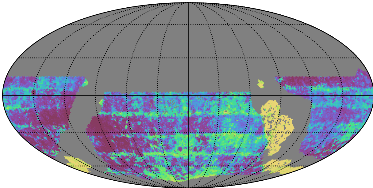
too_combined_s0.5_v3.4_10yrs WFD y band: Median Inter-Night Gap
