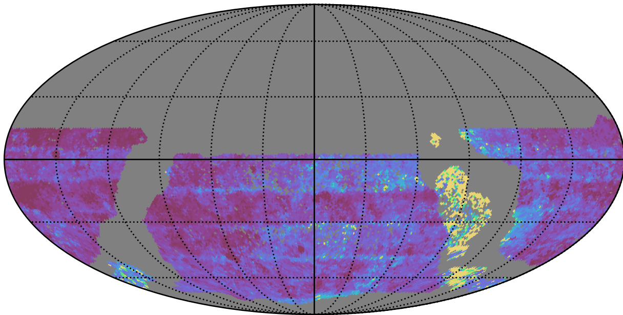
too_combined_s0.5_v3.4_10yrs WFD u band: Median Inter-Night Gap
