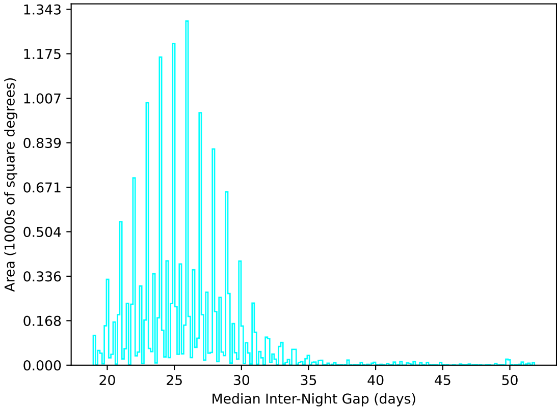
too_combined_s0.5_v3.4_10yrs WFD u band: Median Inter-Night Gap
