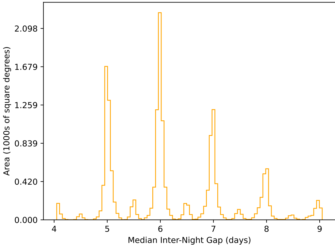
too_combined_s0.5_v3.4_10yrs WFD r band: Median Inter-Night Gap
