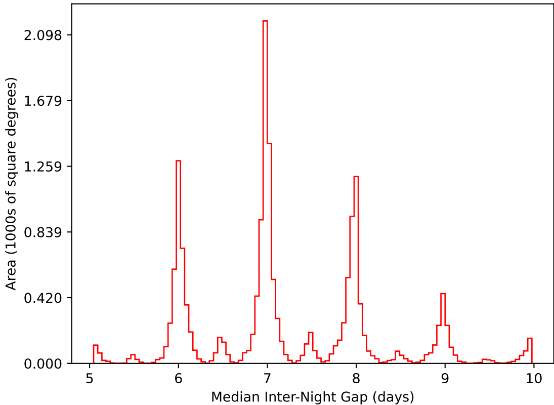
too_combined_s0.5_v3.4_10yrs WFD i band: Median Inter-Night Gap
