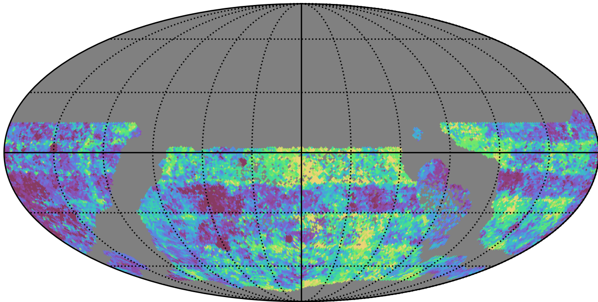
too_combined_s0.5_v3.4_10yrs WFD g band: Median Inter-Night Gap
