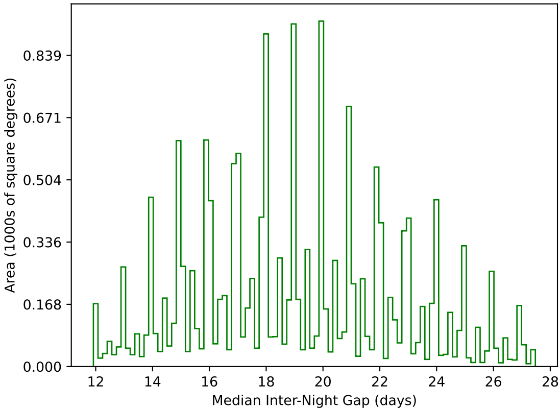
too_combined_s0.5_v3.4_10yrs WFD g band: Median Inter-Night Gap
