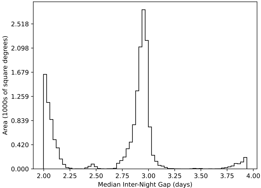
too_combined_s0.5_v3.4_10yrs WFD all bands: Median Inter-Night Gap
