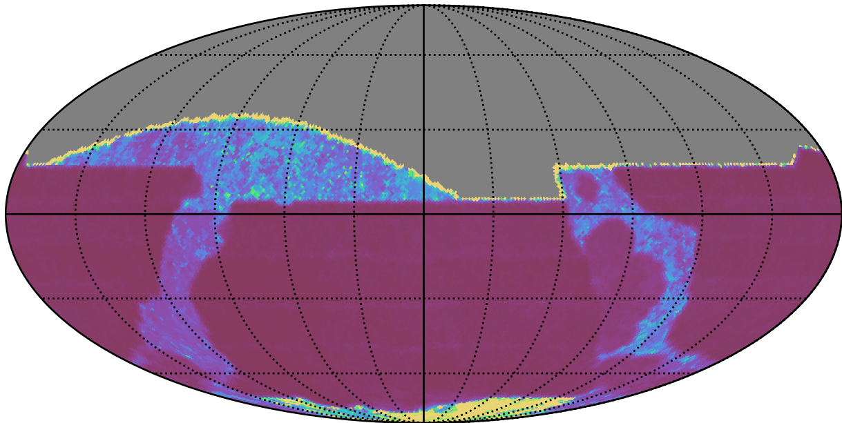
too_combined_s0.5_v3.4_10yrs All sky z band: Median Inter-Night Gap
