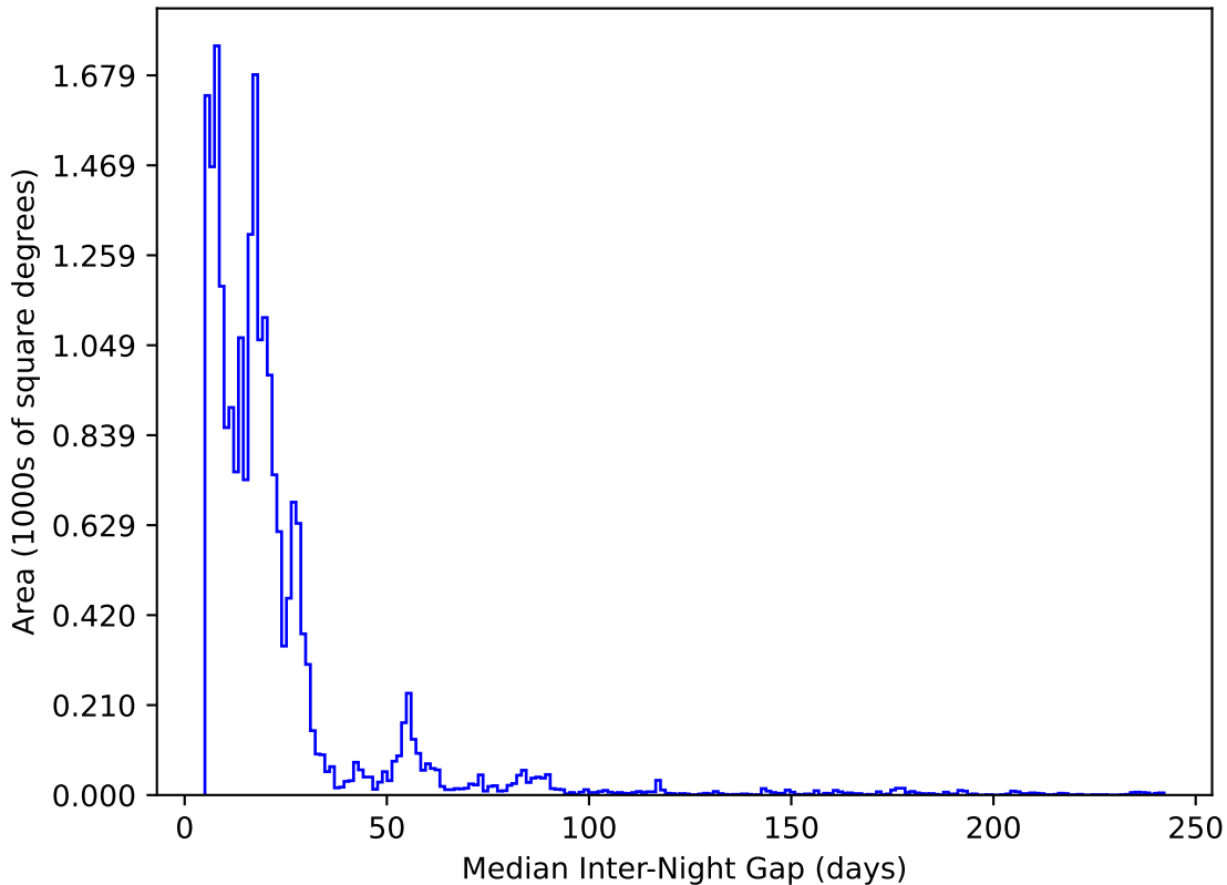
too_combined_s0.5_v3.4_10yrs All sky y band: Median Inter-Night Gap
