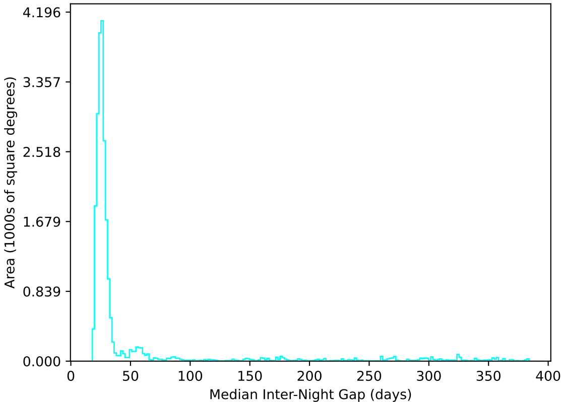
too_combined_s0.5_v3.4_10yrs All sky u band: Median Inter-Night Gap
