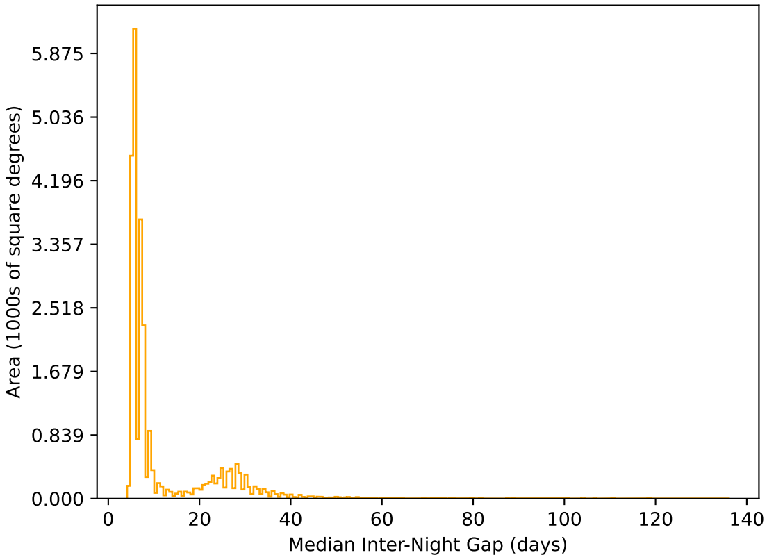
too_combined_s0.5_v3.4_10yrs All sky r band: Median Inter-Night Gap
