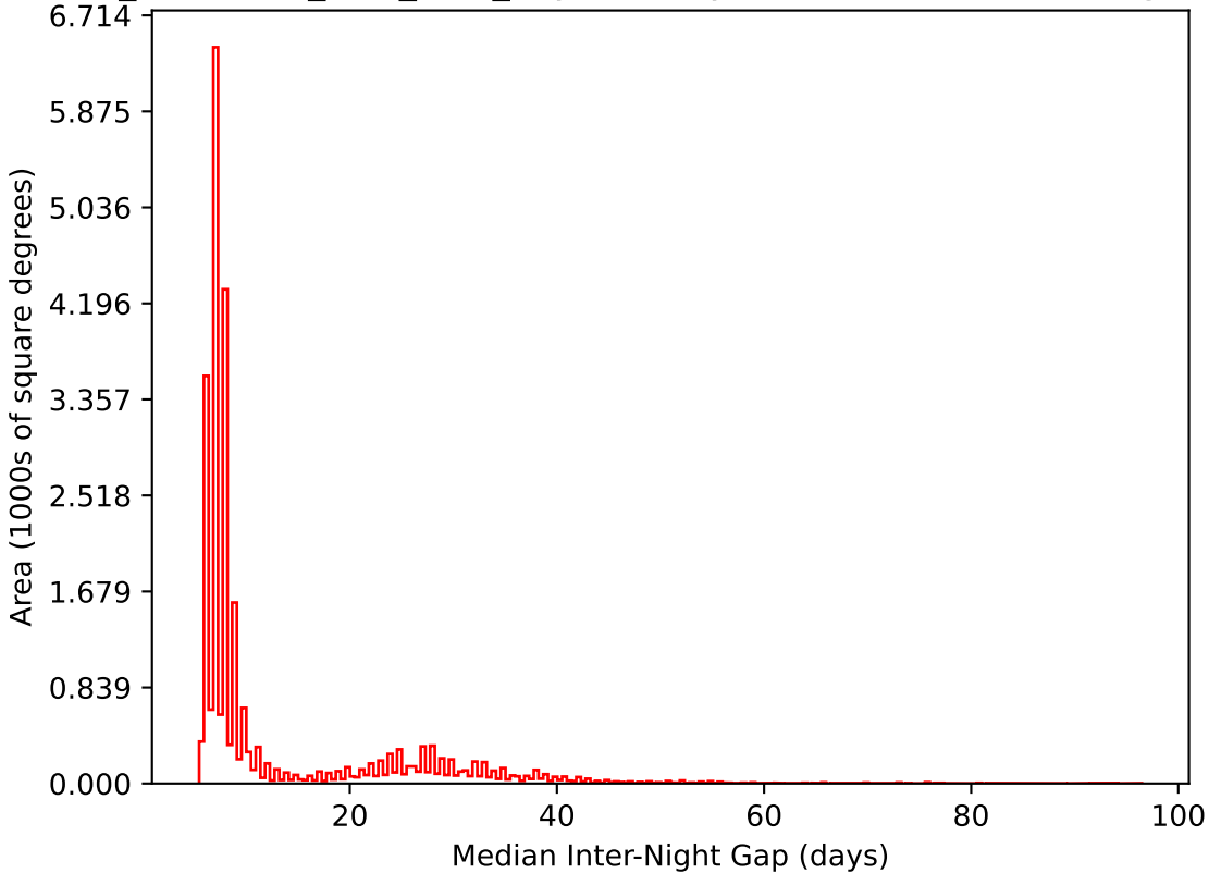
too_combined_s0.5_v3.4_10yrs All sky i band: Median Inter-Night Gap
