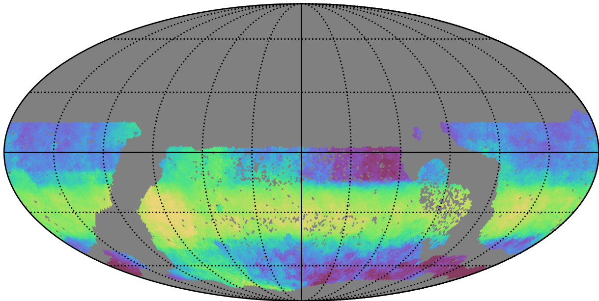
too_combined_s0.5_v3.4_10yrs WFD z band: Median HA
