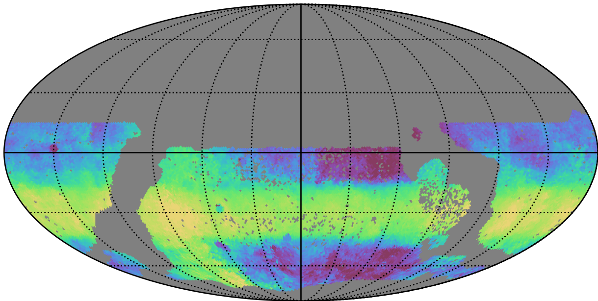
too_combined_s0.5_v3.4_10yrs WFD y band: Median HA
