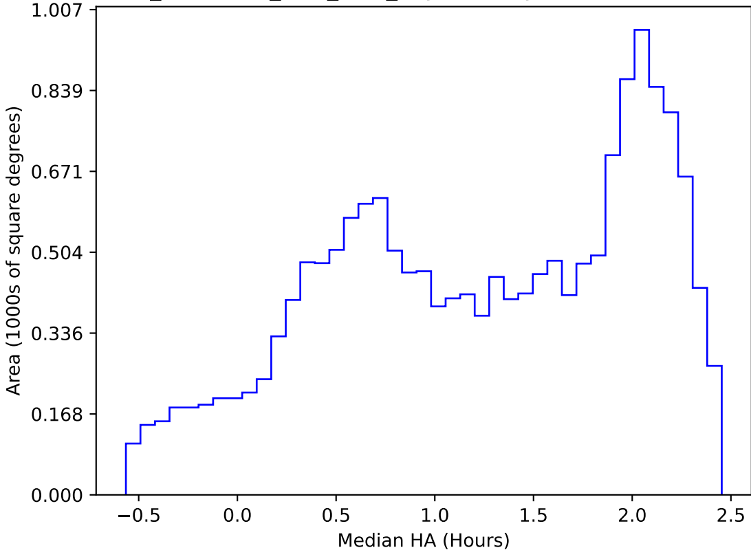
too_combined_s0.5_v3.4_10yrs WFD y band: Median HA
