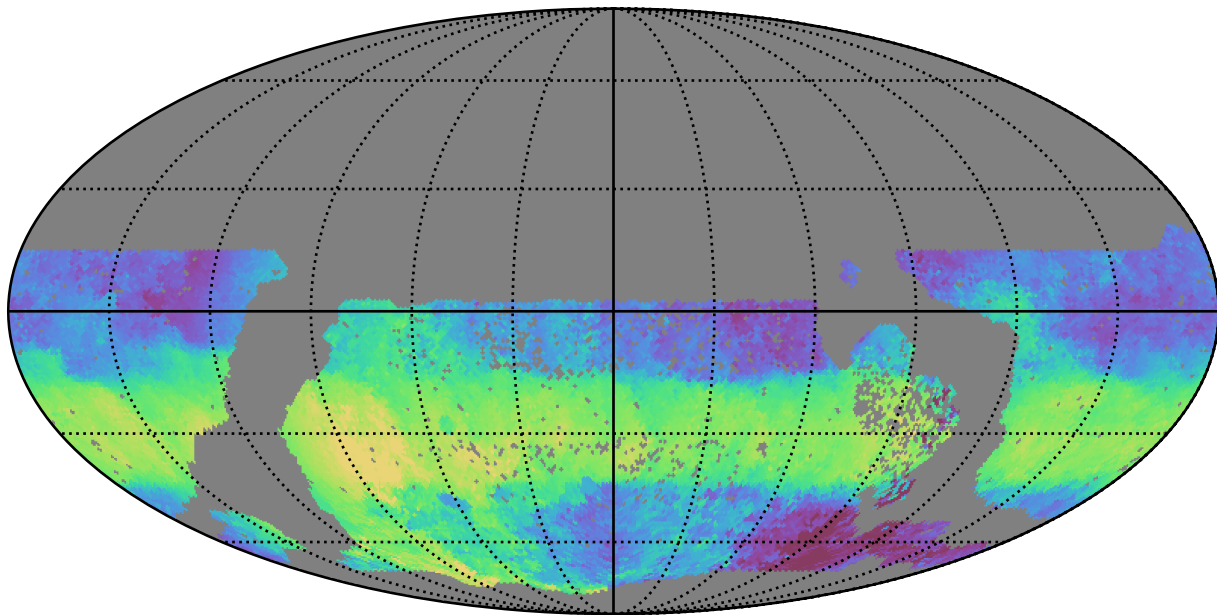
too_combined_s0.5_v3.4_10yrs WFD u band: Median HA
