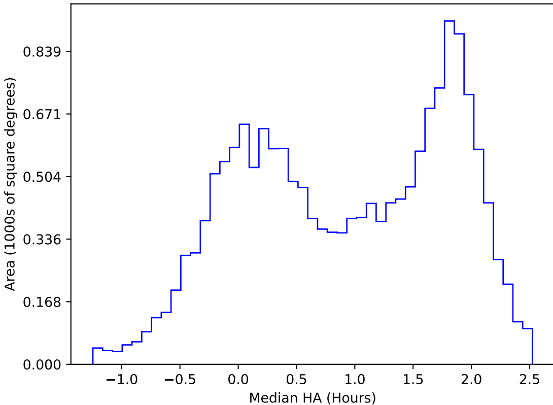
too_combined_s0.5_v3.4_10yrs WFD u band: Median HA
