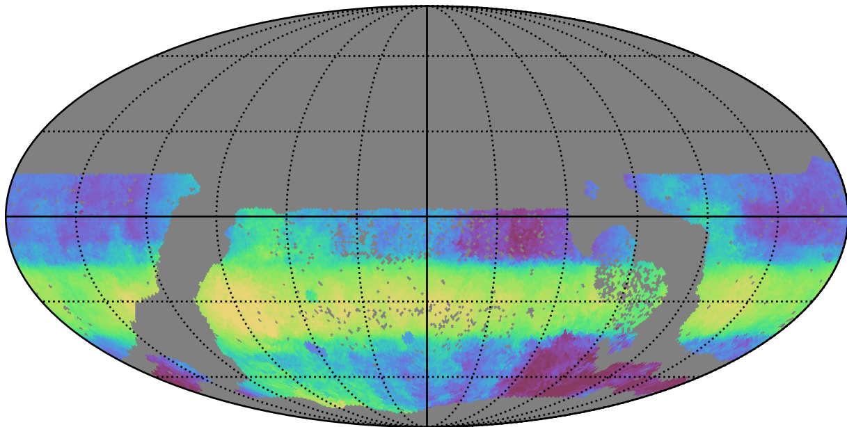
too_combined_s0.5_v3.4_10yrs WFD r band: Median HA
