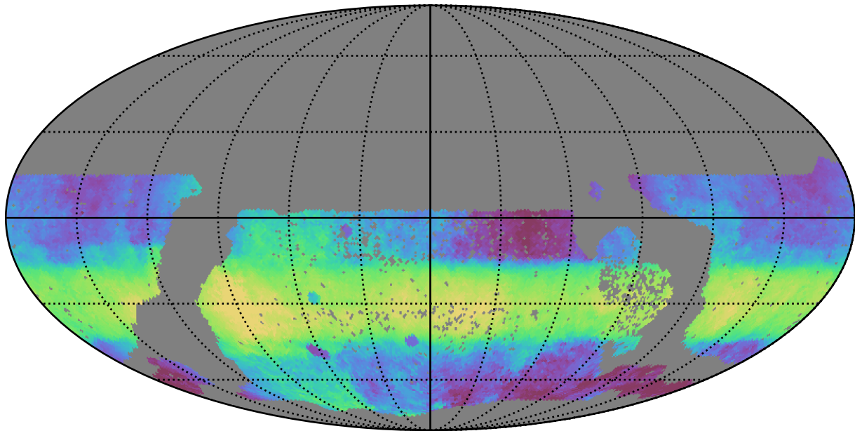
too_combined_s0.5_v3.4_10yrs WFD i band: Median HA
