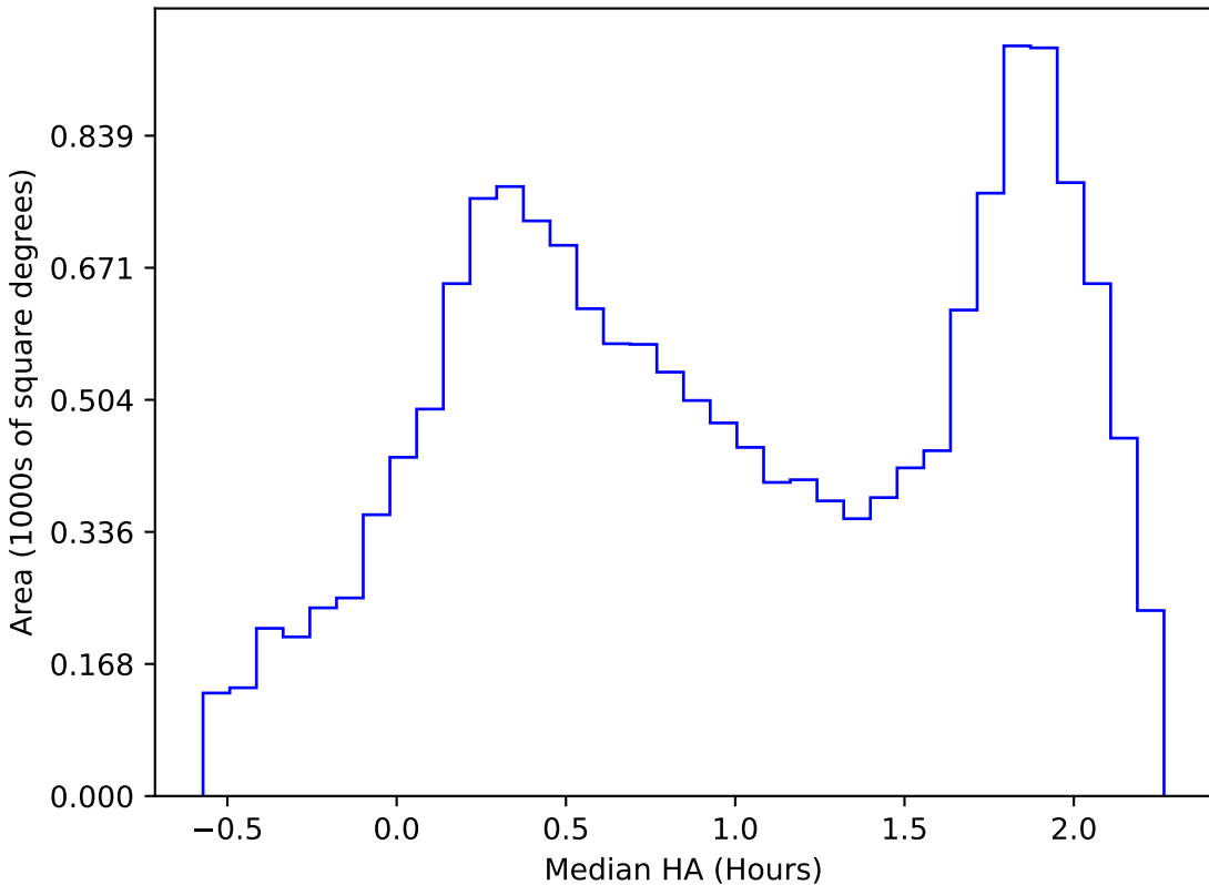
too_combined_s0.5_v3.4_10yrs WFD i band: Median HA
