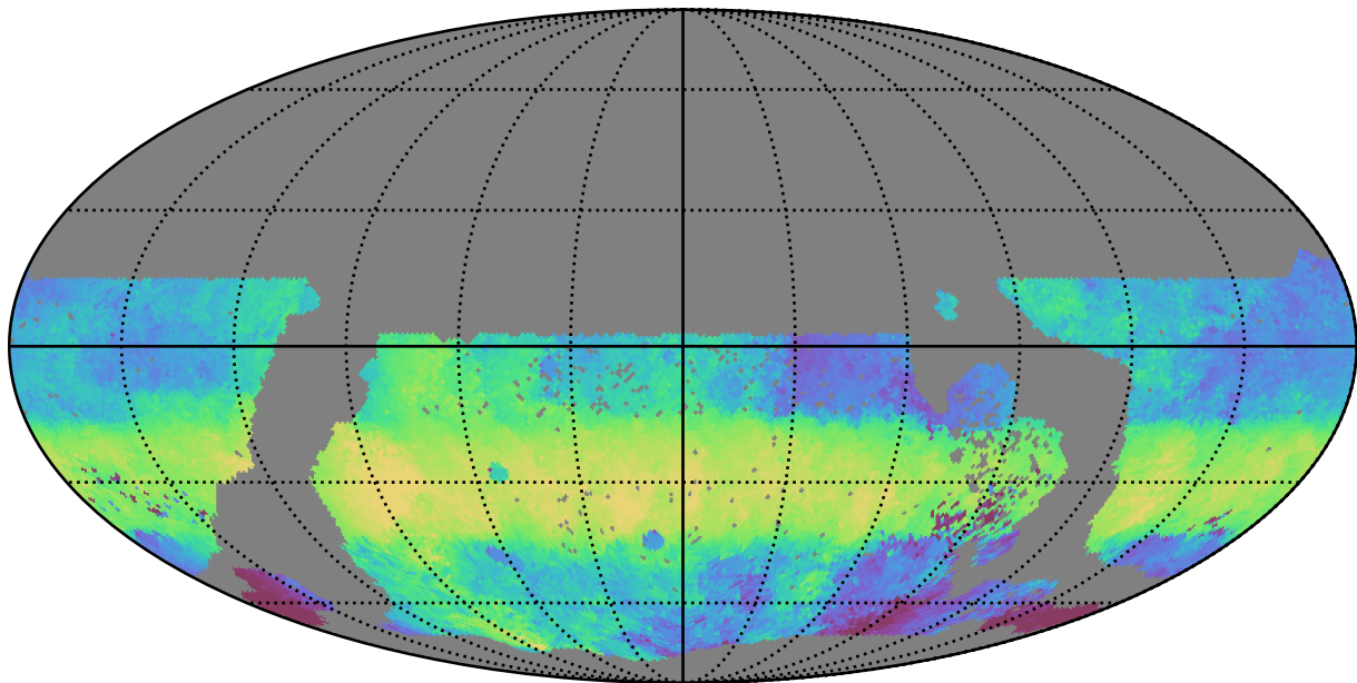
too_combined_s0.5_v3.4_10yrs WFD g band: Median HA
