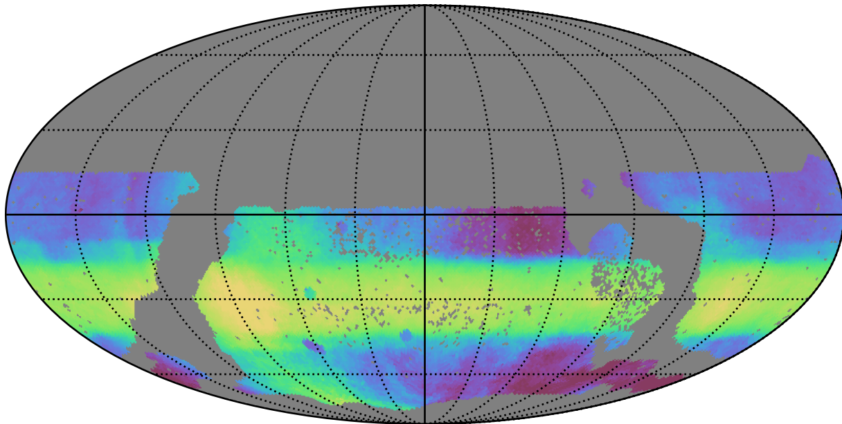
too_combined_s0.5_v3.4_10yrs WFD all bands: Median HA
